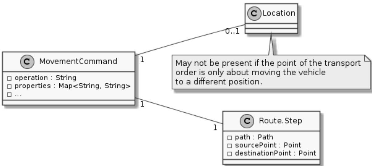
Figure 6. MovementCommand-related classes
